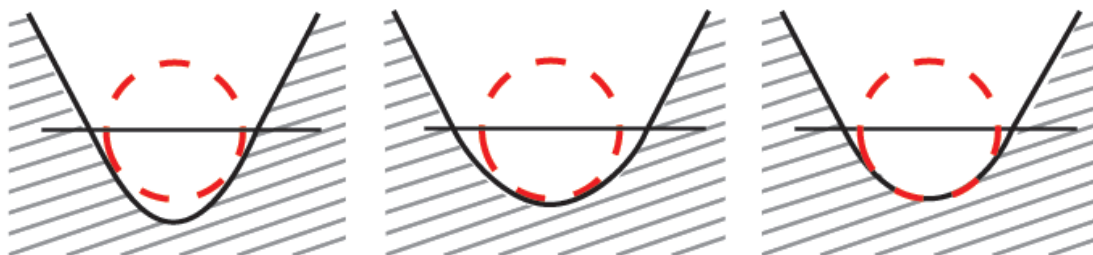
Figure 3-3 Rolling and twisting of a rope resulting from the fleet angle
