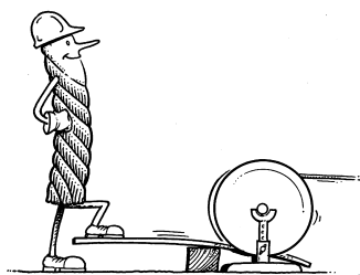
Figure 2-6 - Installing rope under tension, about 10% of the nominal rope pull
